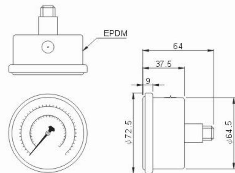
AE-AB/25 . AE-ABK/25 . BE-AB/25
