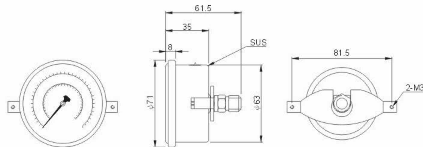
AE-AU/25 . AE-AUK/25 . BE-AU/25
