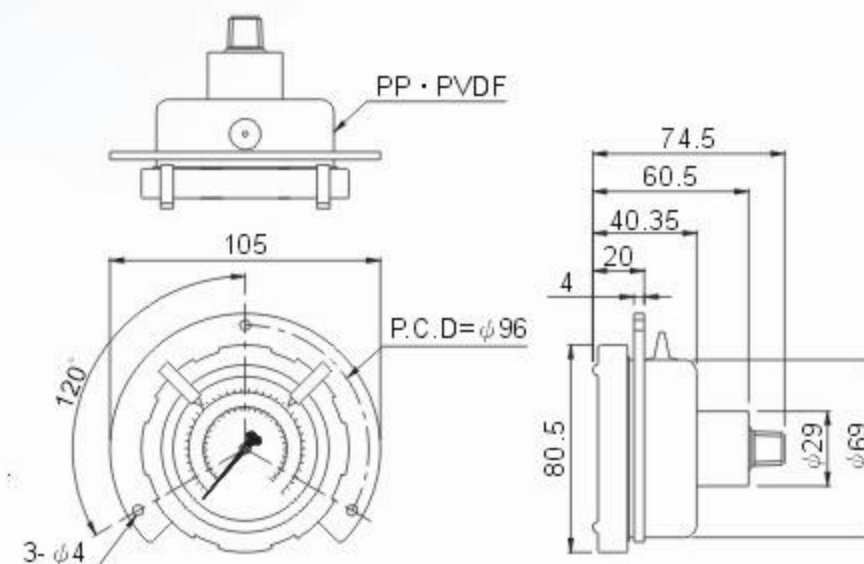
AF-AF/25 . AF-AFK/25 . BF-AF/25
