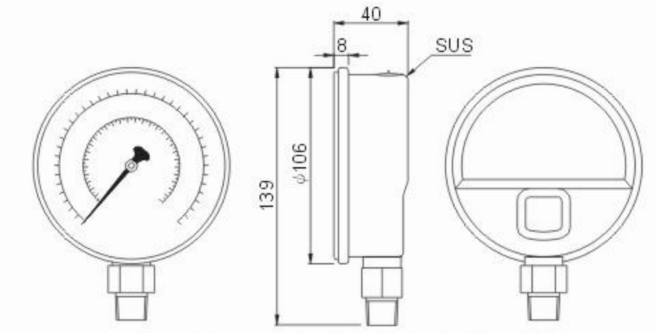
AC-A/4 . AC-AK/4 . BC-A/4
