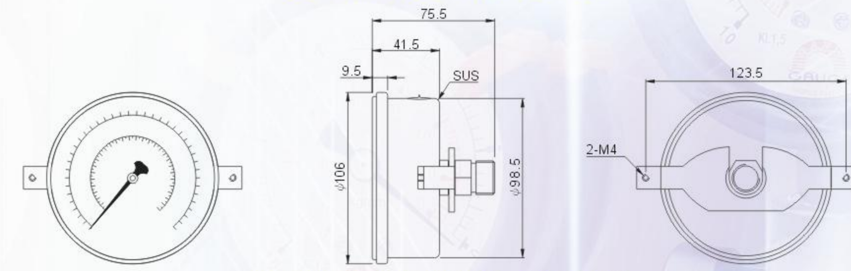
AE-AU/4 . AE-AUK/4 . BE-AU/4
