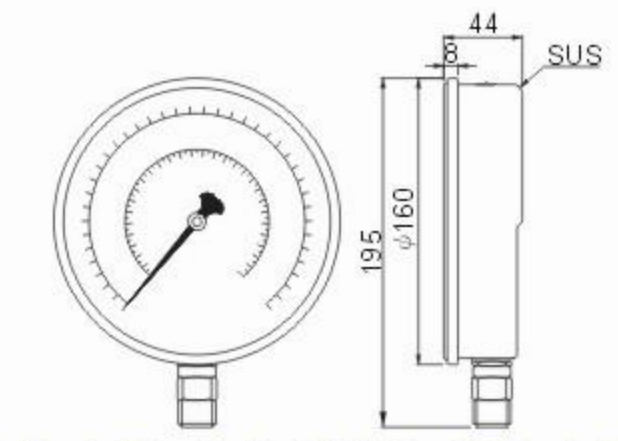
AC-A/6 . AC-AK/6 . BC-A/6
